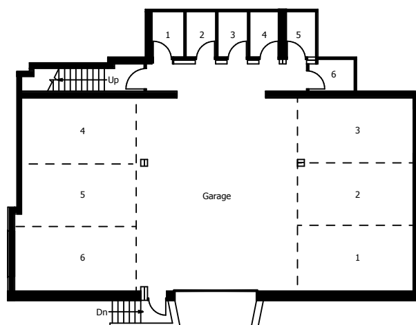
Lower Ground Floor Parking and Stores
